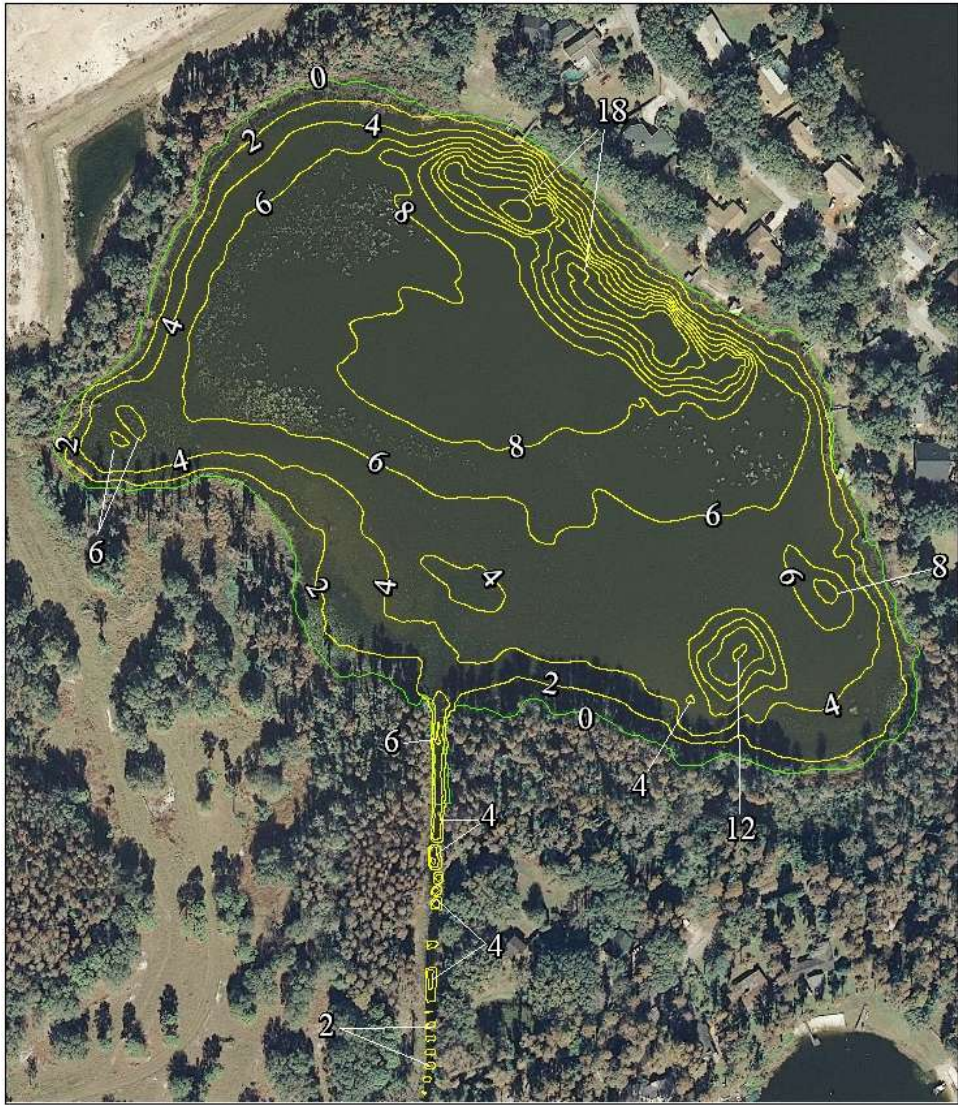
Figure 2. 2011 2-Foot Bathymetric Contour Map for Lake Virginia
