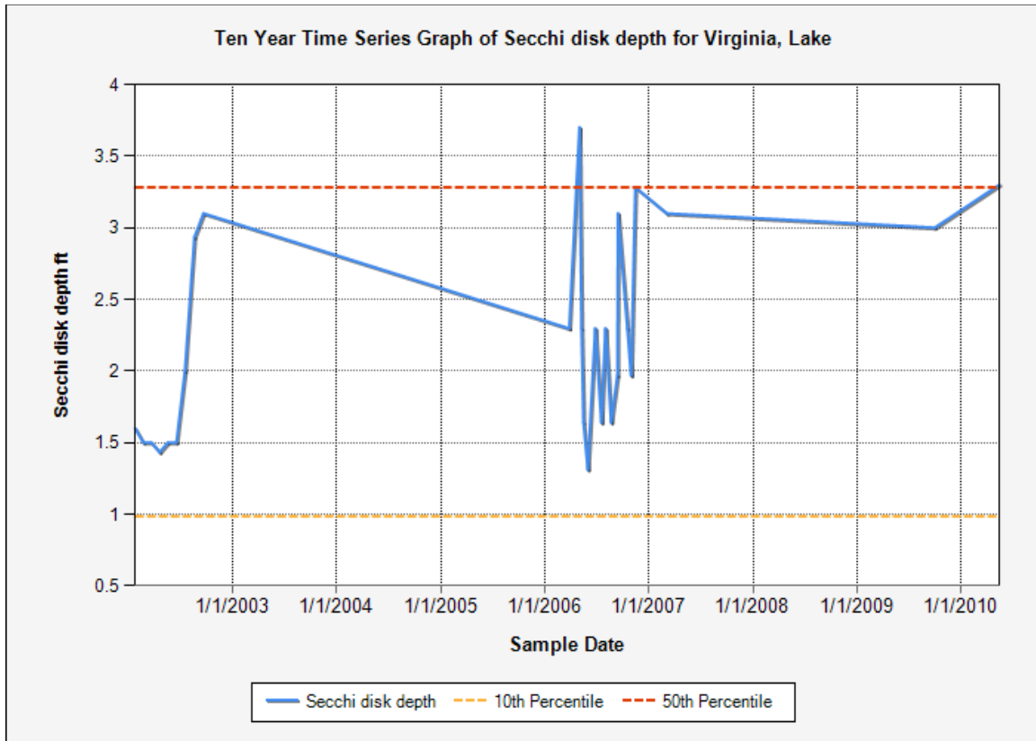
Figure 9. Recent Secchi Disk graph for Lake Virginia viii
