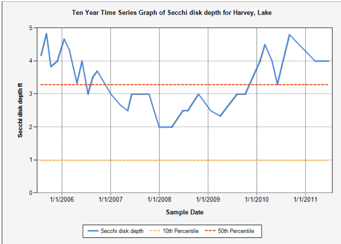
Figure 9. Recent Secchi Disk graph for Lake Harvey viii
