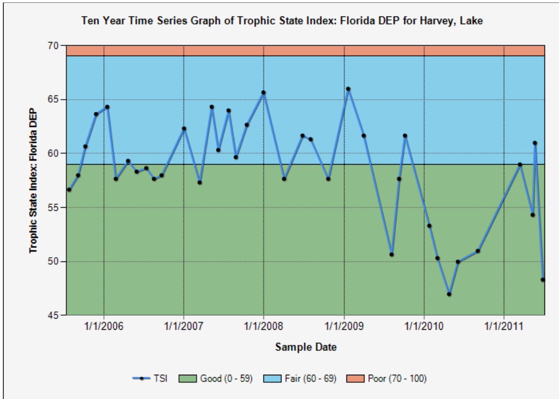
Figure 7. Recent Trophic State Index (TSI) graph for Lake Harvey vi
