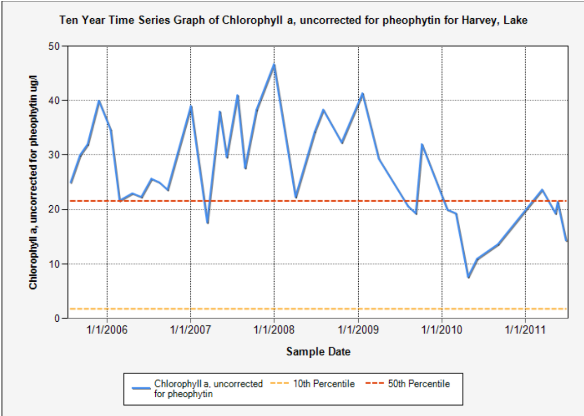
Figure 8. Recent Chlorophyll a graph for Lake Harvey vii
