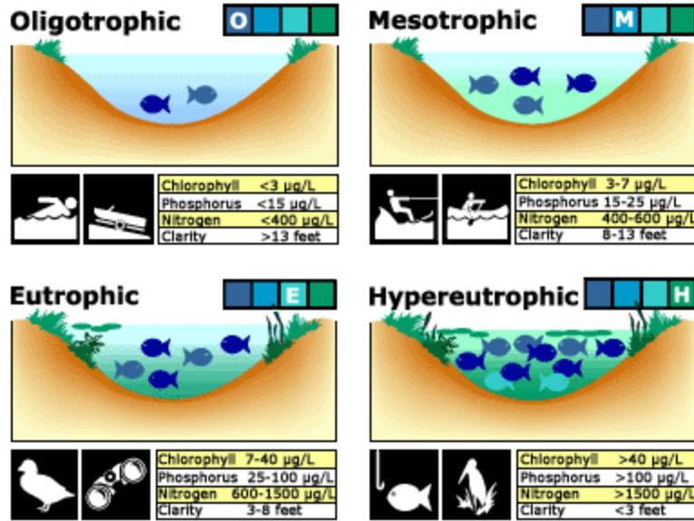
Figure 9. Tropic States
