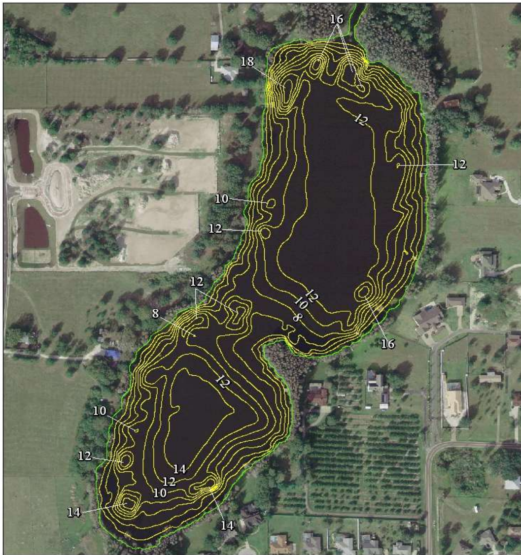
Figure 1. Contour map for Lake Kell. The mapping technique used in 2009 employs a standard DGPS for horizontal position and a fathometer for depth.
