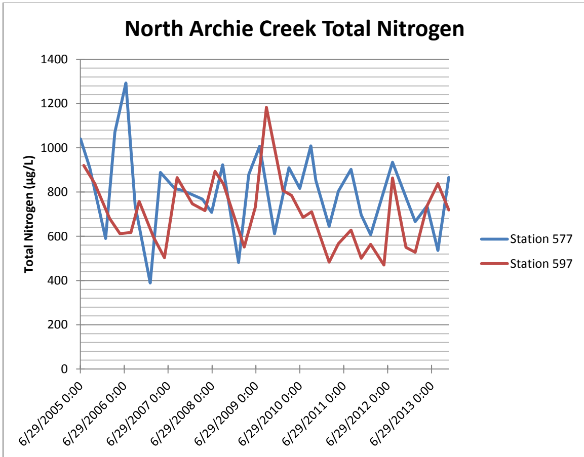
Figure 8 Total Nitrogen sample values for two North Archie Creek Stations 2011-2013
