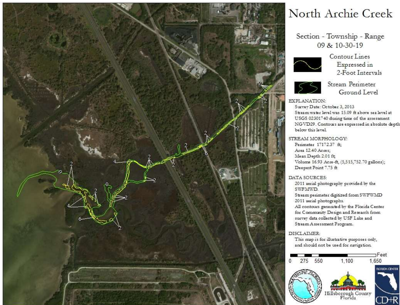
Figure 2. 2013 2-Foot Bathymetric Map for North Archie Creek
