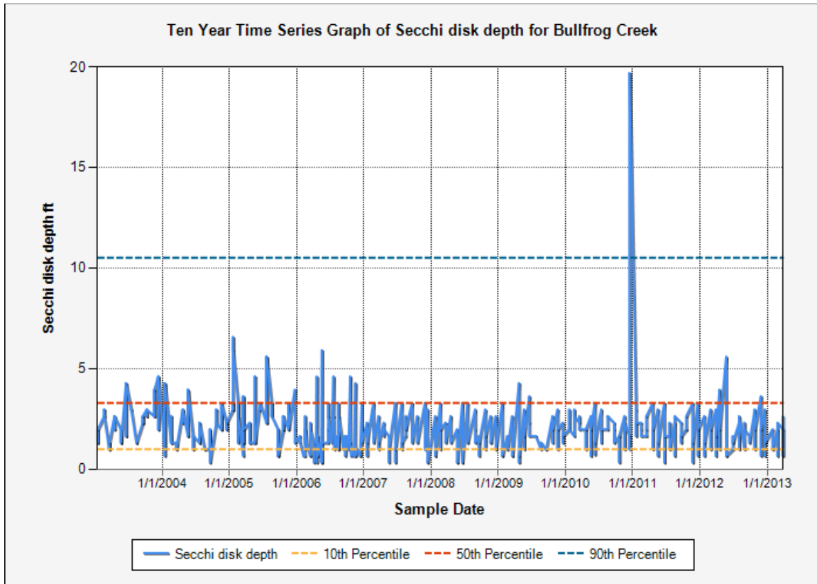
Figure 17. Recent Secchi Disk graph for Bullfrog Creek ix
