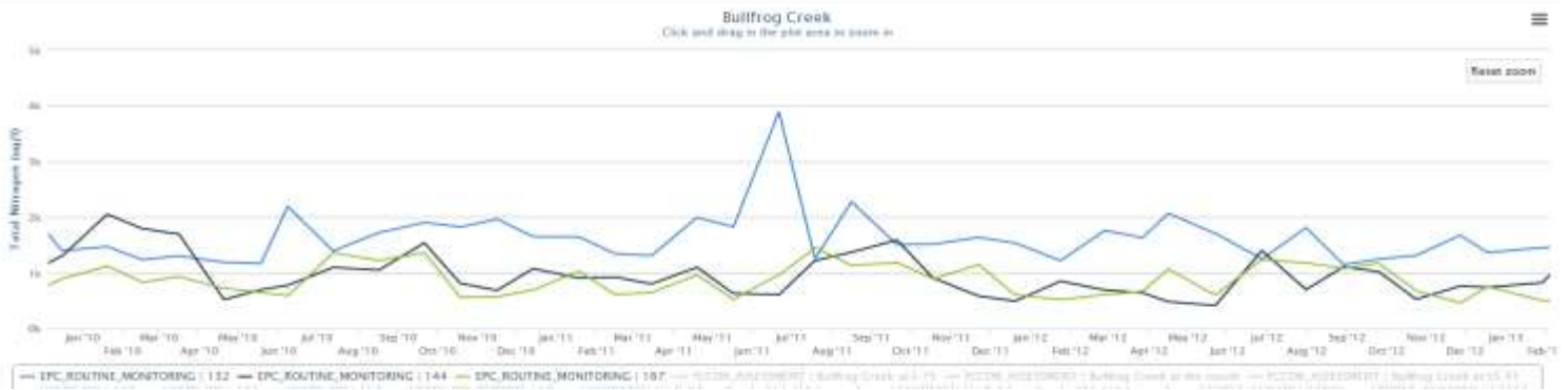
Figure 20 Total Nitrogen sample values for three Bullfrog Creek Stations 2010-2012
