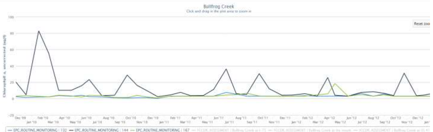
Figure 19 Chlorophyll a sample values for three Bullfrog Creek stations 2010-2012
