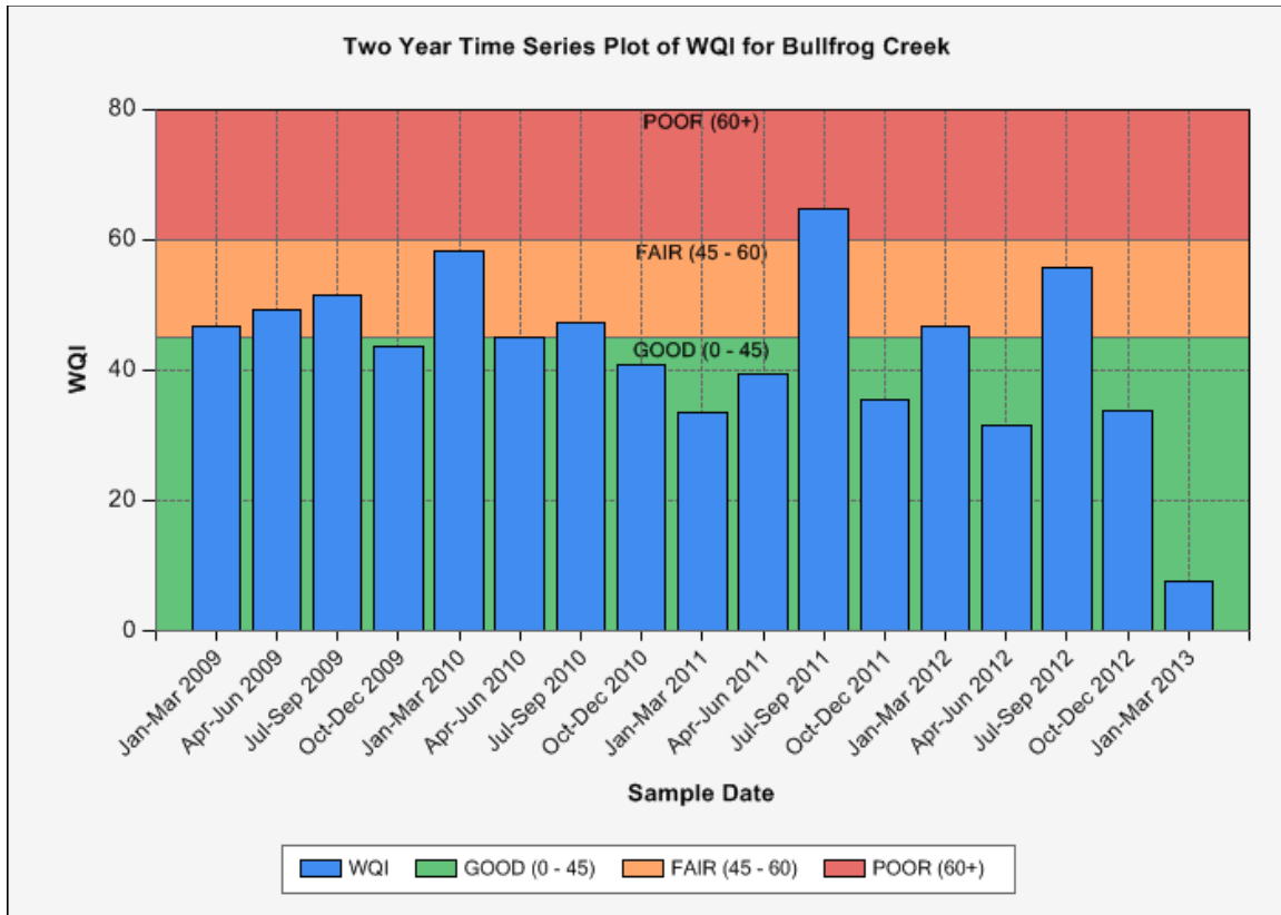
Figure 15. Recent Water Quality Index (WQI) graph for Bullfrog Creek vii
