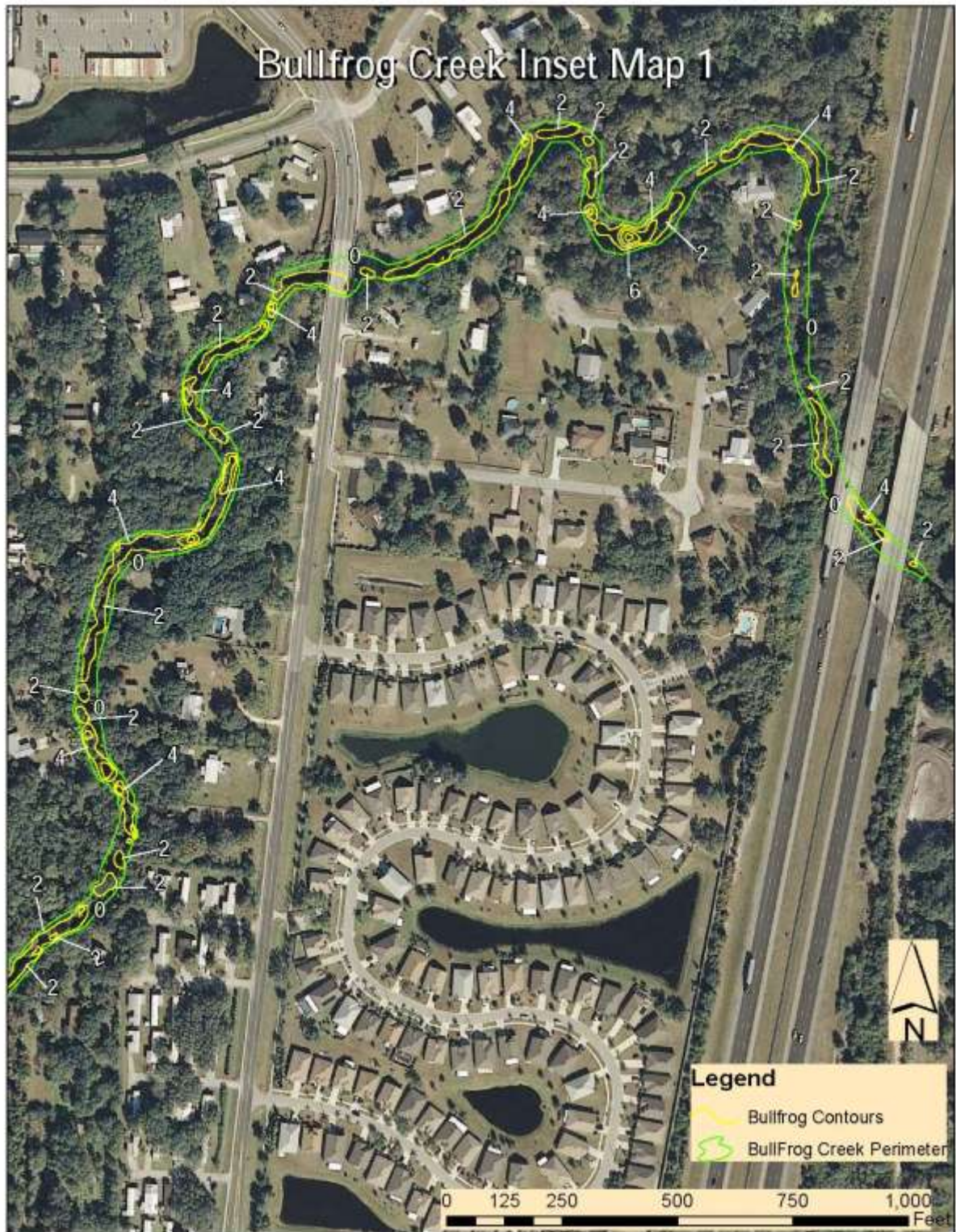
Figure 3 Bullfrog Creek 2012 Bathymetric Contour Inset Map 1
