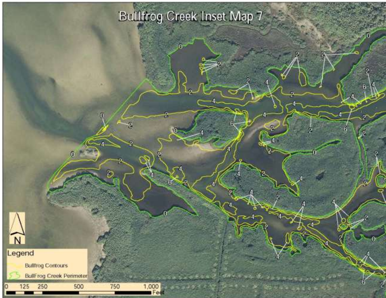
Figure 9 Bullfrog Creek 2012 Bathymetric Contour Inset Map 7
