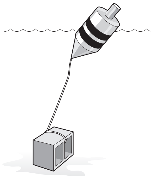
Figure 7-3. The marker buoy. This instrument may be used to identify monitoring sites in sheltered areas of the estuary.
