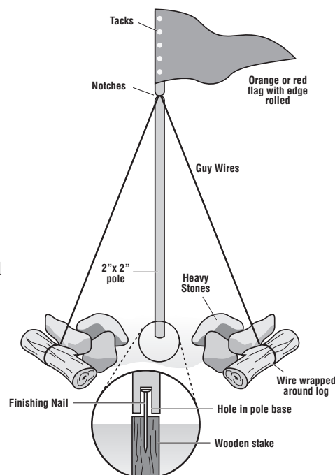
Figure 7-2. Construction of a landmark flag (adapted from Compton, 1962).
